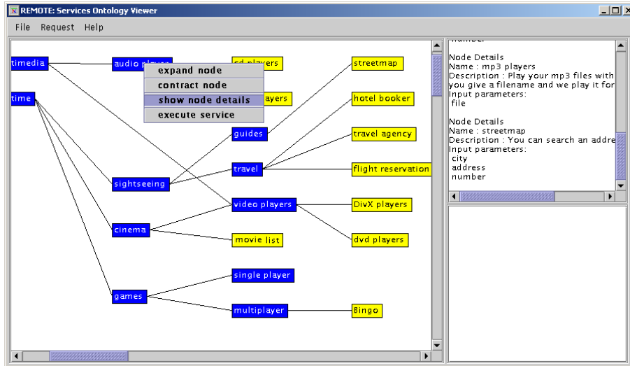
Fig. 4. Service catalog retrieved for the keywords specified in Figure 3
