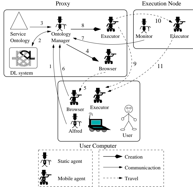
Fig. 1. Agents in REMOTE
