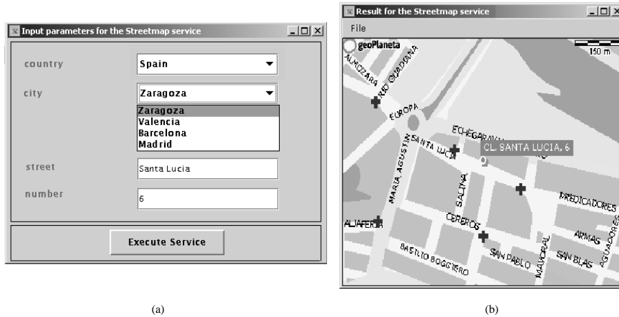
Fig. 5. (a) Input parameter GUI for the streetmap service and (b) result obtained after remote execution
