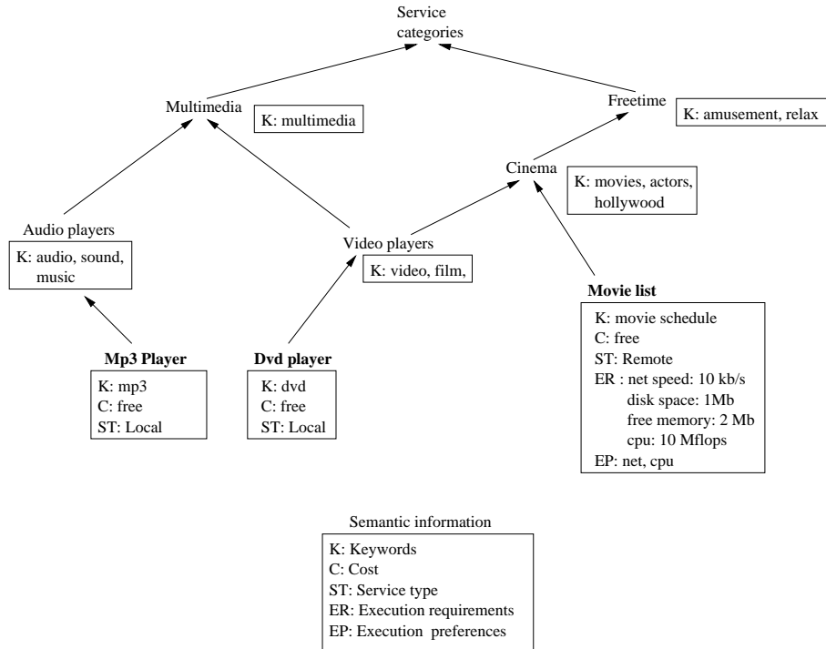
Fig. 2. Extract of the ontology used by REMOTE and terms definitions
