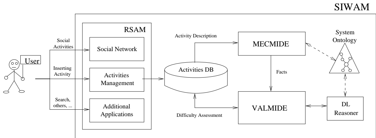
Figure 1: Architecture of SIWAM.
