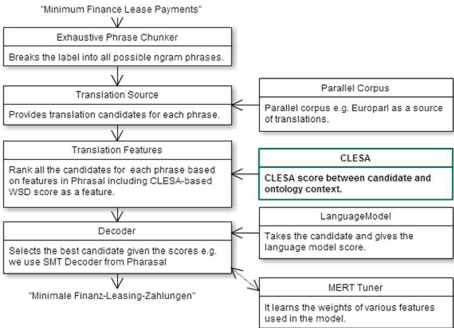
Figure 1: Phrase-based SMT architecture with CLESA integration.
