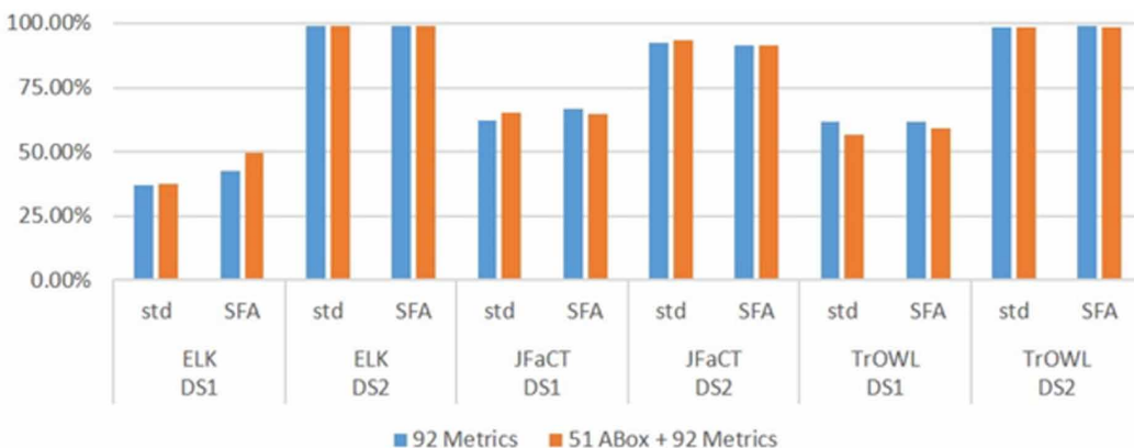
Figure 3. Comparison of R^2 values in 10-fold Cross Validation procedure
